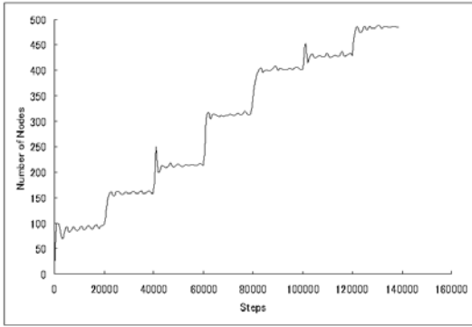
Fig. 4. Number of nodes during incremental learning (Environment I – Environment VII)
